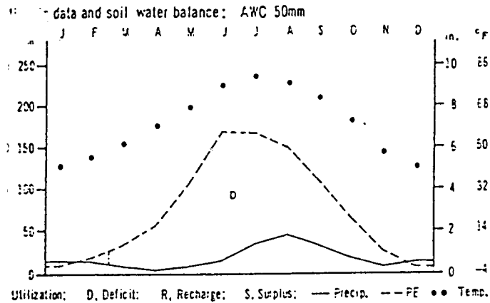
Figure 9.—Climatic data and soil water balance for a soil that has an aridic (torric) soil moisture regime.
