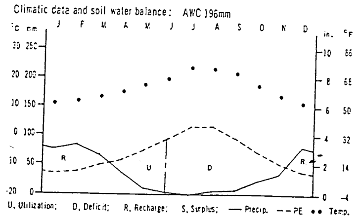
Figure 13.—Climatic data and soil water balance for a soil that has a xeric soil moisture regime.
