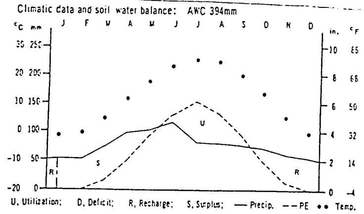
Figure 10.—Climatic data and soil water balance for a soil that has a udic soil moisture regime.
