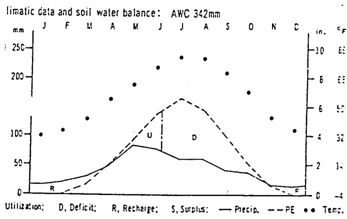
Figure 12.—Climatic data and soil water balance for a soil that has an ustic soil moisture regime.
